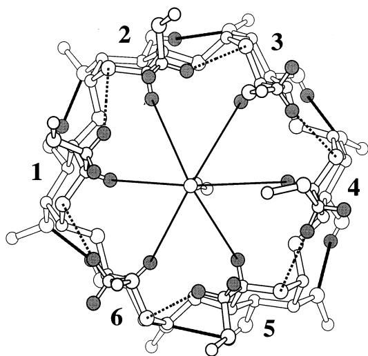
Fig. 2. 'Round' macrocyclic conformation of DIMEA is stabilized by intramolecular, interglucose \text{O}-3-\text{H}(n)\cdots\text{O}-2(n+1) and \text{C}-6-\text{H}(n)\cdots\text{O}-5(n+1) hydrogen bonds as shown with thick solid and dashed lines, respectively. The acetonitrile is held in position at the central cavity of DIMEA by \text{C}-5-\text{H}\cdots\text{N} interactions (thin solid lines). For clarity, hydrogen atoms \text{C}-5-\text{H} , \text{C}-6-\text{H}_2 , and \text{O}-3-\text{H} are shown as small spheres; C atoms are medium-sized spheres; and O and N atoms are large spheres.
