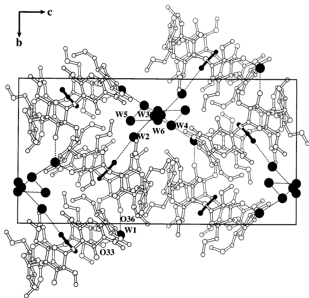
Fig. 3. Crystal packing of the inclusion complex DIMEA- \text{CH}_3\text{CN}\cdot 2\text{H}_2\text{O} . Acetonitrile and water molecules are drawn with filled bonds and circles. Dashed lines indicate possible hydrogen bonds within a distance of 3.6 Å of O and N atoms, respectively. W-1 is fully and W-2–W-6 are partially (0.15–0.25) occupied. The latter are located in an infinite channel formed by methyl groups (see Fig. 4).
